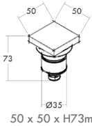
50 x 50 x H73mm
