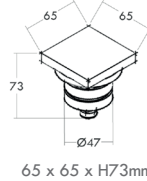
65 x 65 x H73mm
