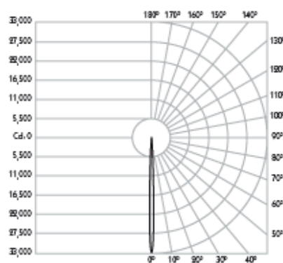
Product Photometry tested in accordance with LM-79 at 3000K, please enquire for 2700K data.
