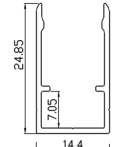
A4115.1217.CLH Aluminium Clip High 25mm
