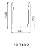
A4115.1217.CLP Plastic Clip 25mm
