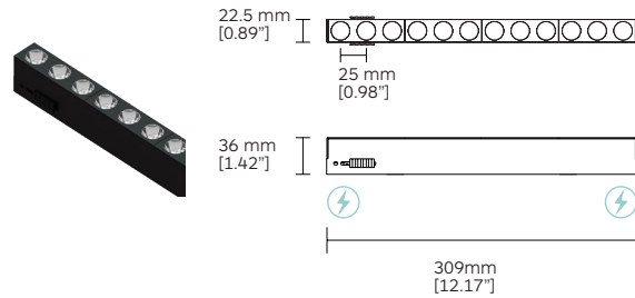
G145 Min. L= 309mm (12.17"), 12 x LED, 1 Link
