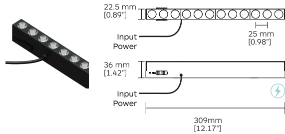
G146 Min. L= 309mm (12.17"), 12 x LED, 1 Link
